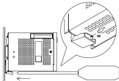
Figure 3.3. Removing a unit from a DIN rail with a phillips-head screwdriver < 1 / 3 >
