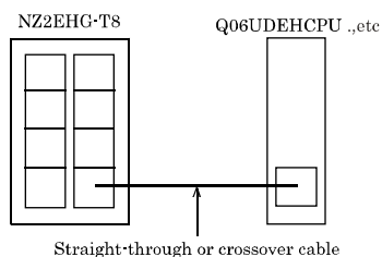
Figure 4.1. Connection example
