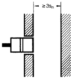
Fig.1: Shielded type (except SUS)
