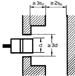
Fig.3: Non-shielded type
